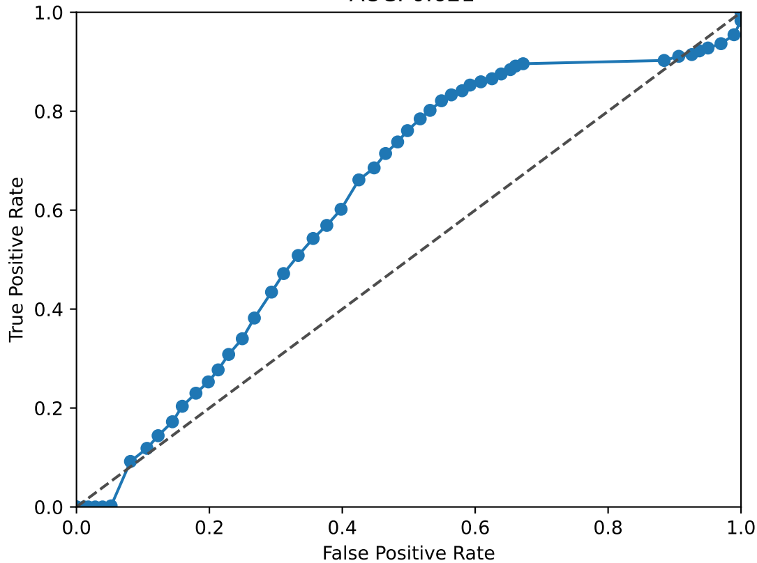
ETS1 ROC Curve AUC: 0.621
