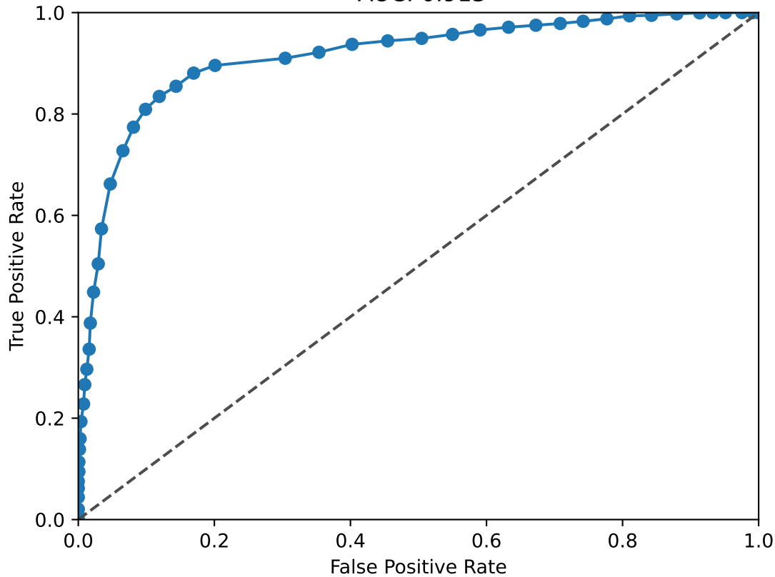
FOS ROC Curve AUC: 0.913
