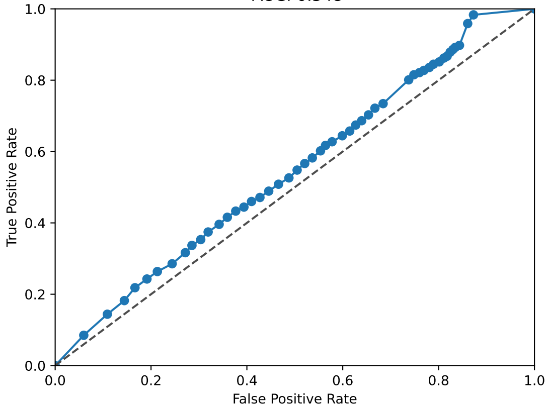
GRHL2 ROC Curve AUC: 0.548
