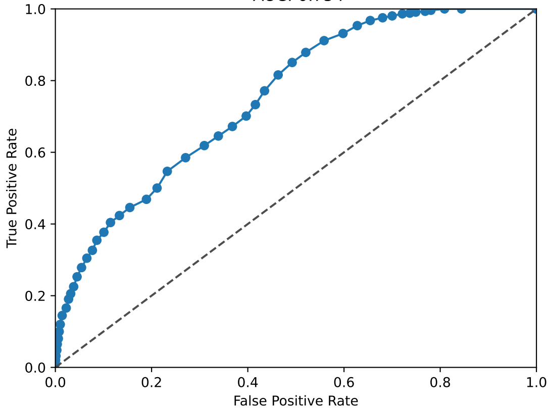
HSF2 ROC Curve AUC: 0.754
