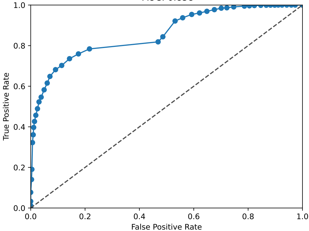
JUNB ROC Curve AUC: 0.858
