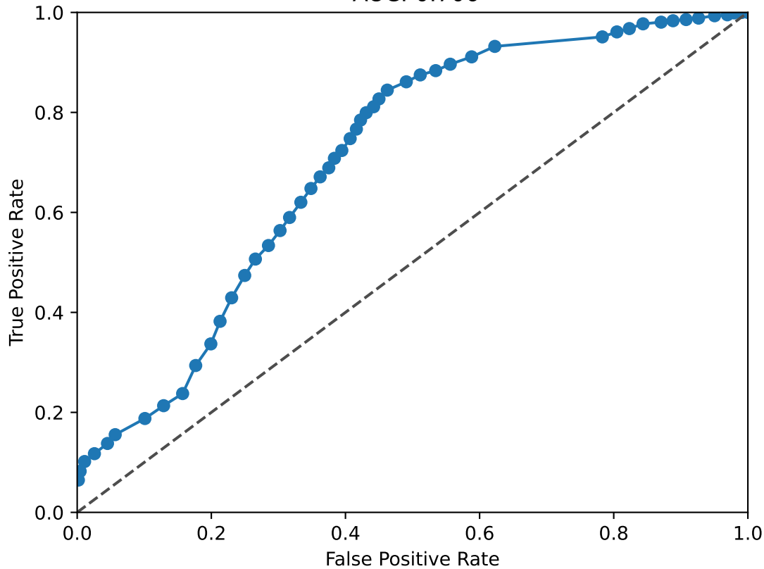
LMX1B ROC Curve AUC: 0.706
