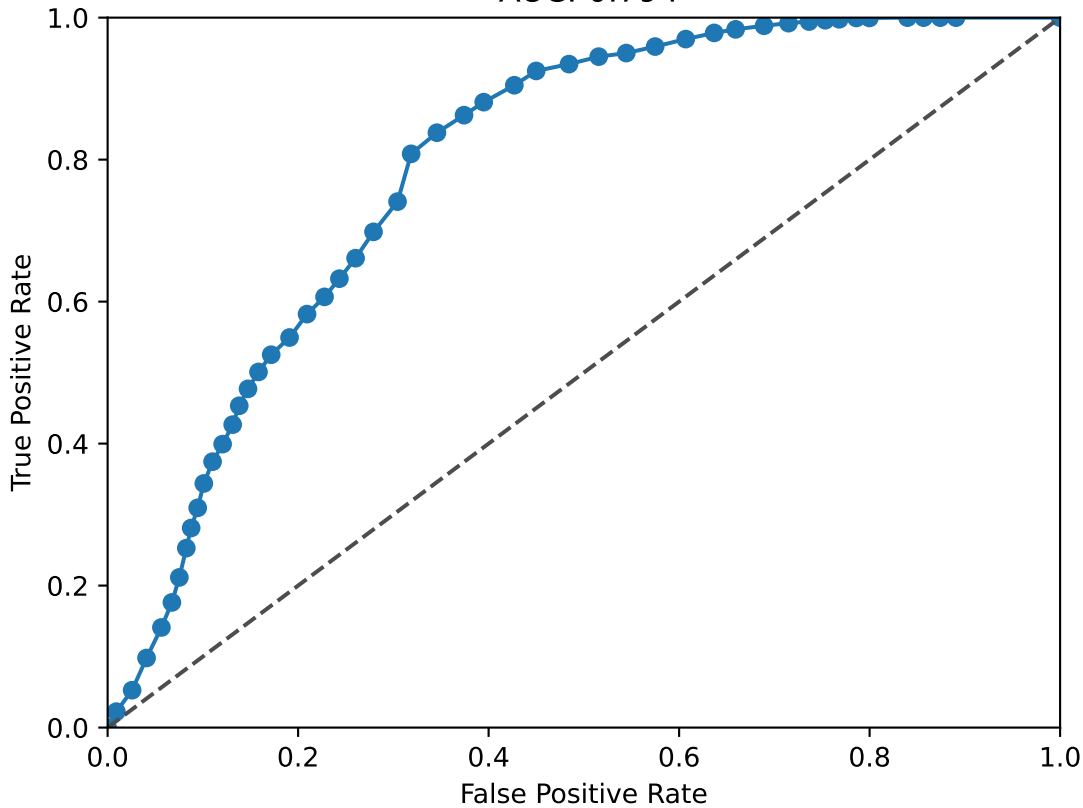
NFIB ROC Curve AUC: 0.794
