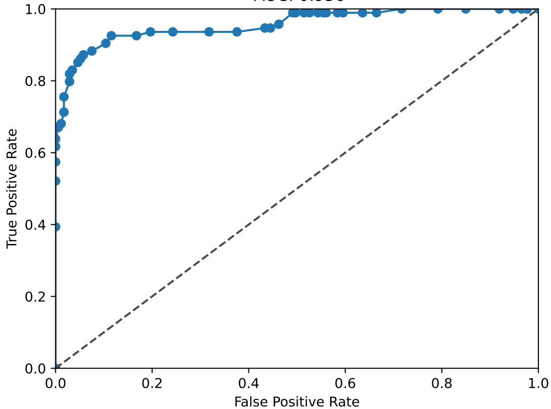
EGR1 ROC Curve AUC: 0.956
