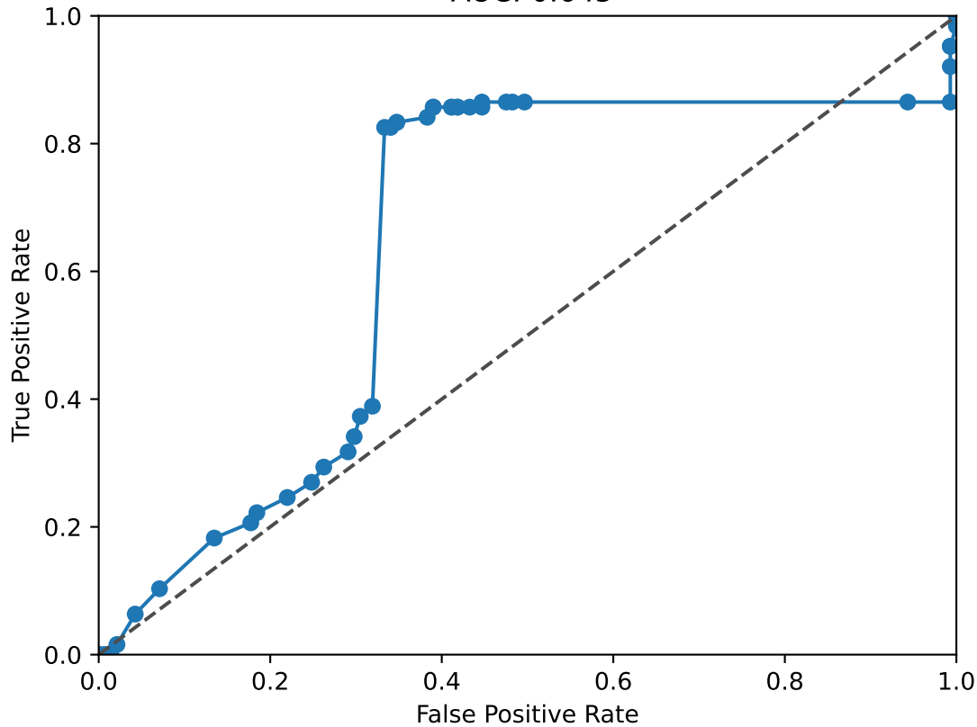
ETS1 ROC Curve AUC: 0.645
