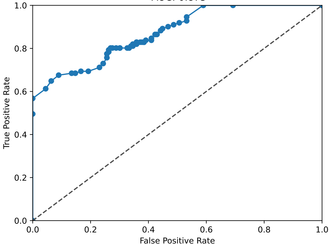
GRHL2 ROC Curve AUC: 0.873
