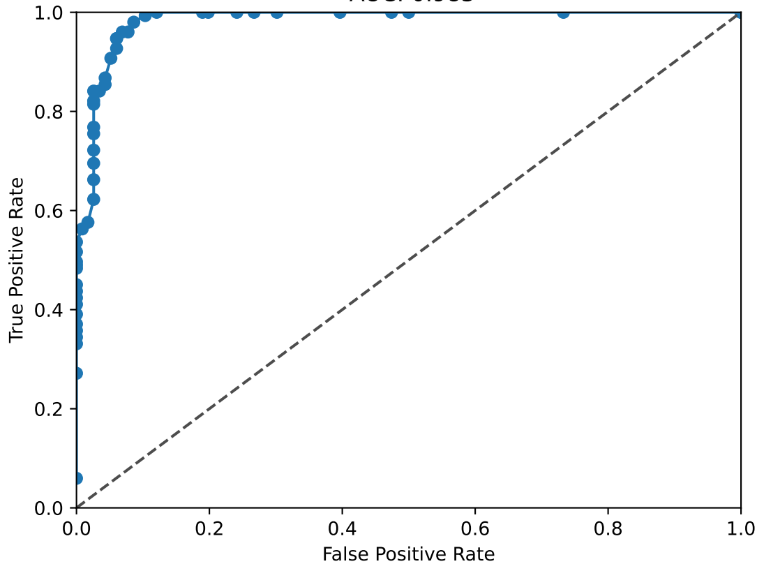
HSF2 ROC Curve AUC: 0.983
