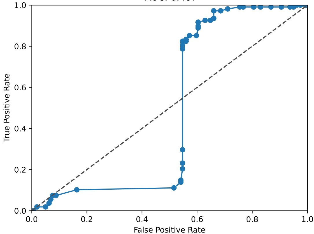
KMT2A ROC Curve AUC: 0.487
