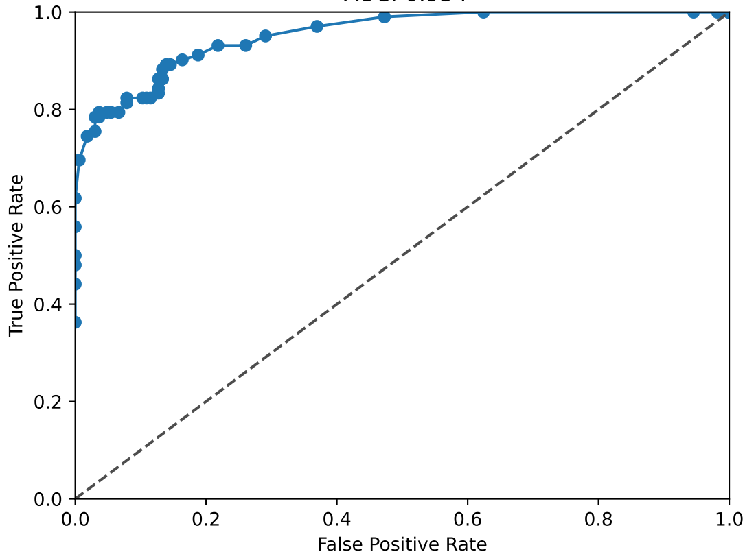
LMX1B ROC Curve AUC: 0.954
