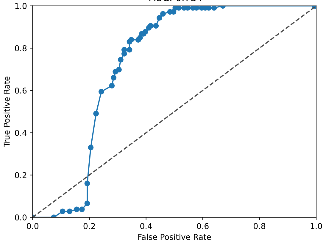
NCAM1 ROC Curve AUC: 0.734
