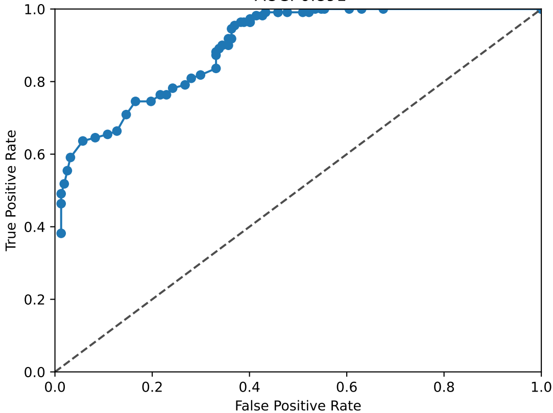
RORA_RORB ROC Curve AUC: 0.891
