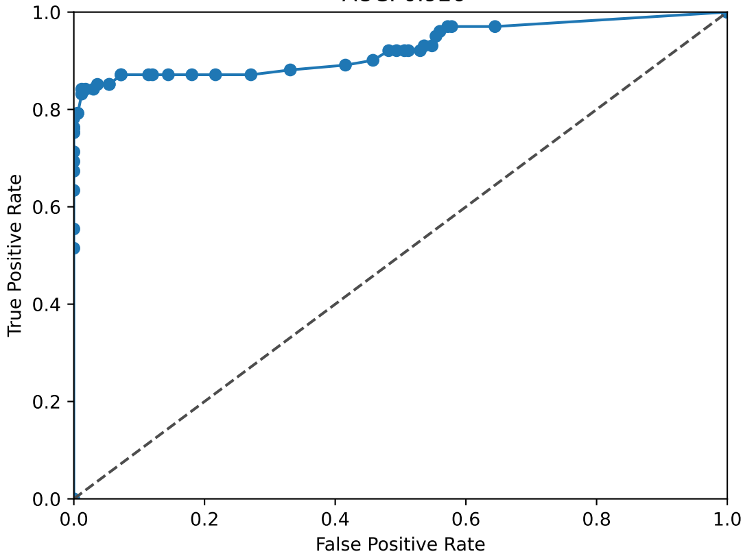
RUNX1 ROC Curve AUC: 0.926
