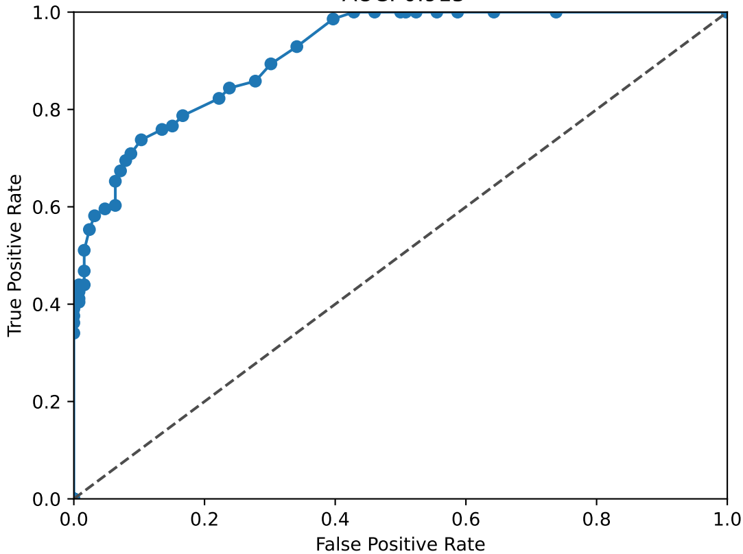
STAT2 ROC Curve AUC: 0.915
