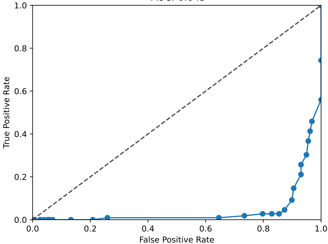
TCF7L2 ROC Curve AUC: 0.045
