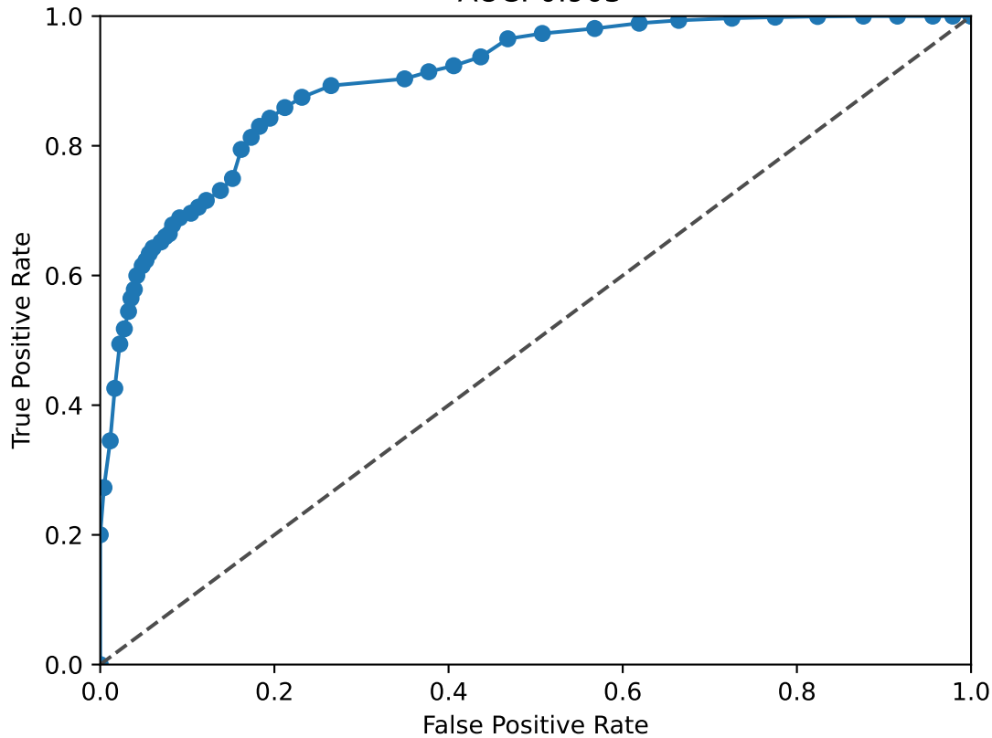
BACH1 ROC Curve AUC: 0.903
