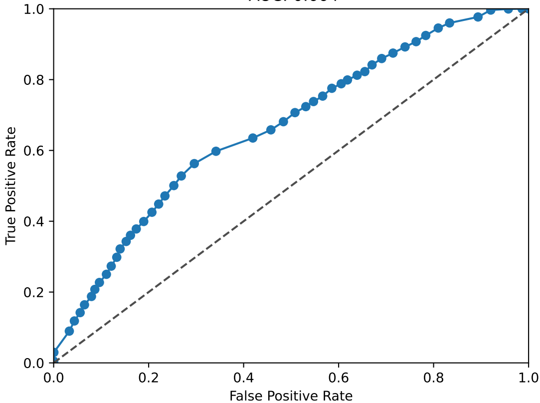
NFIB ROC Curve AUC: 0.664
