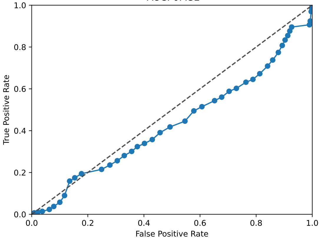
PKNOX2 ROC Curve AUC: 0.432
