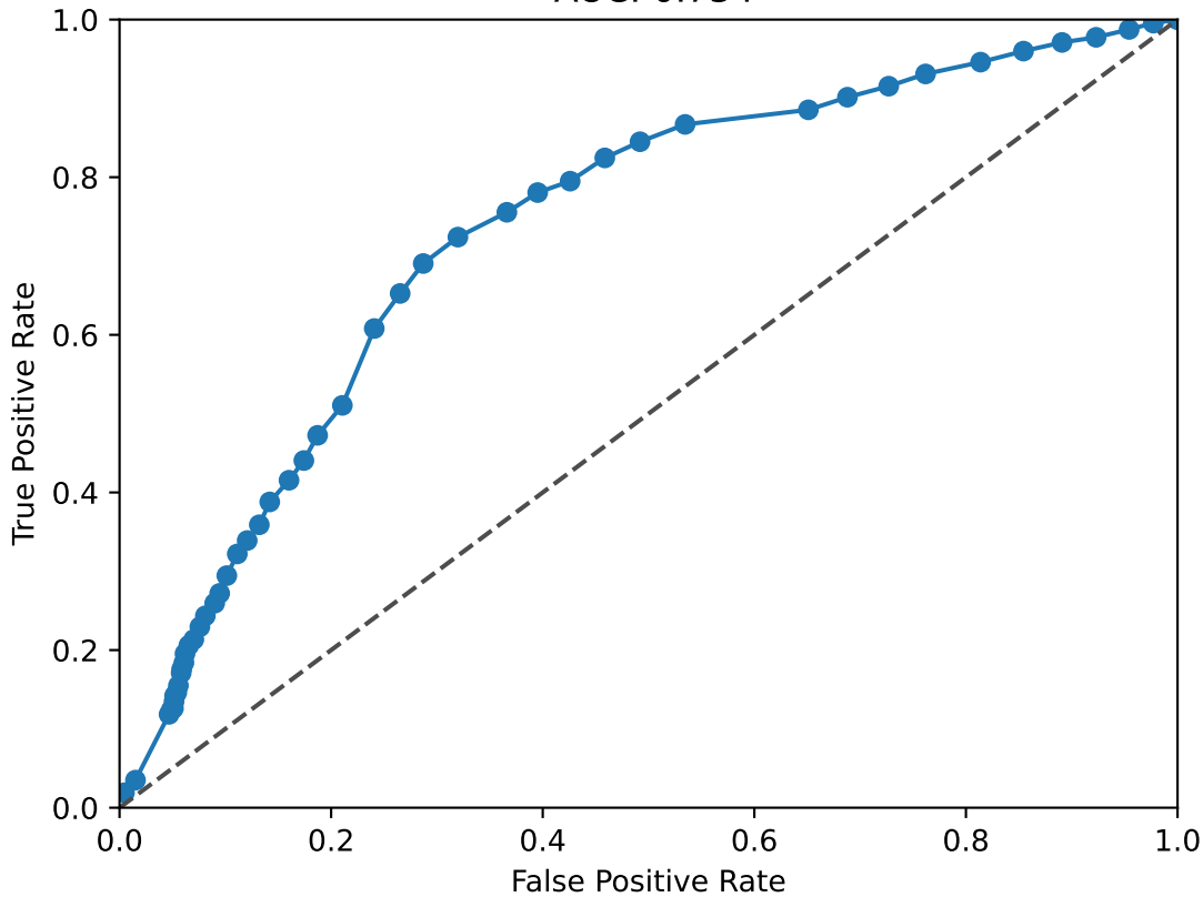
TCF7L1 ROC Curve AUC: 0.734
