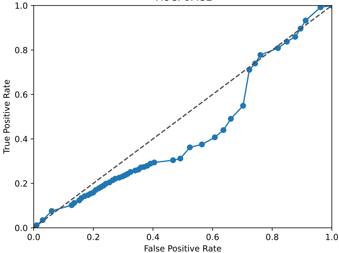
TCF7L2 ROC Curve AUC: 0.432
