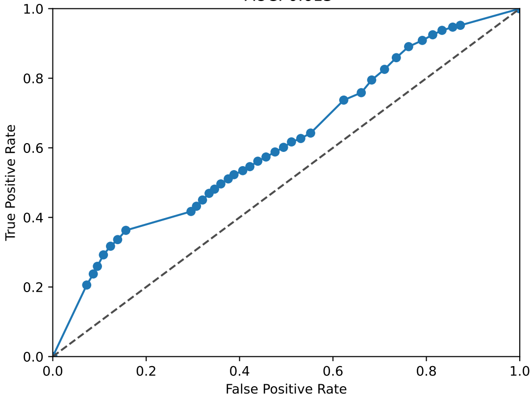
EHF ROC Curve AUC: 0.613
