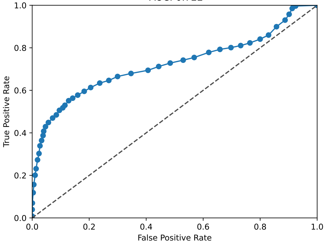
RUNX1 ROC Curve AUC: 0.722
