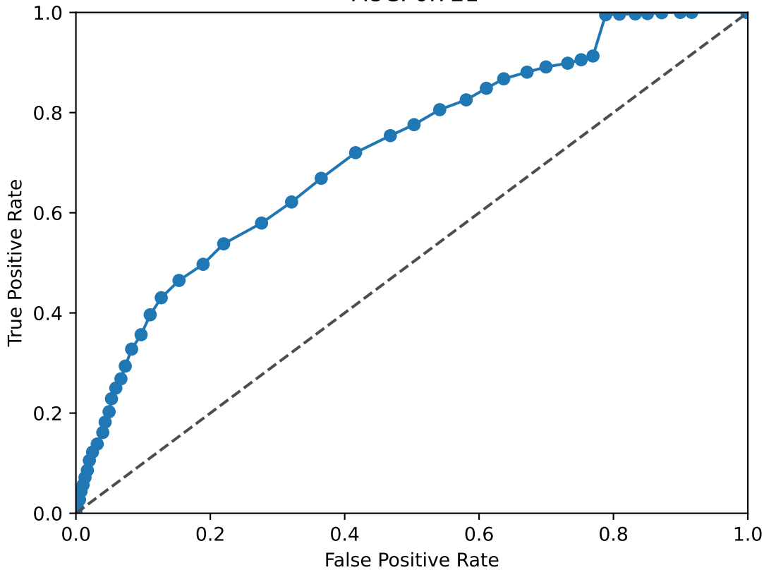
SIX4 ROC Curve AUC: 0.721
