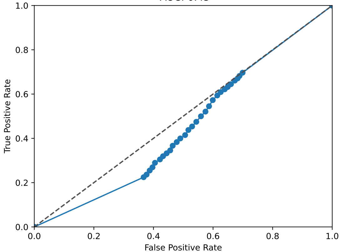
THR B ROC Curve AUC: 0.45
