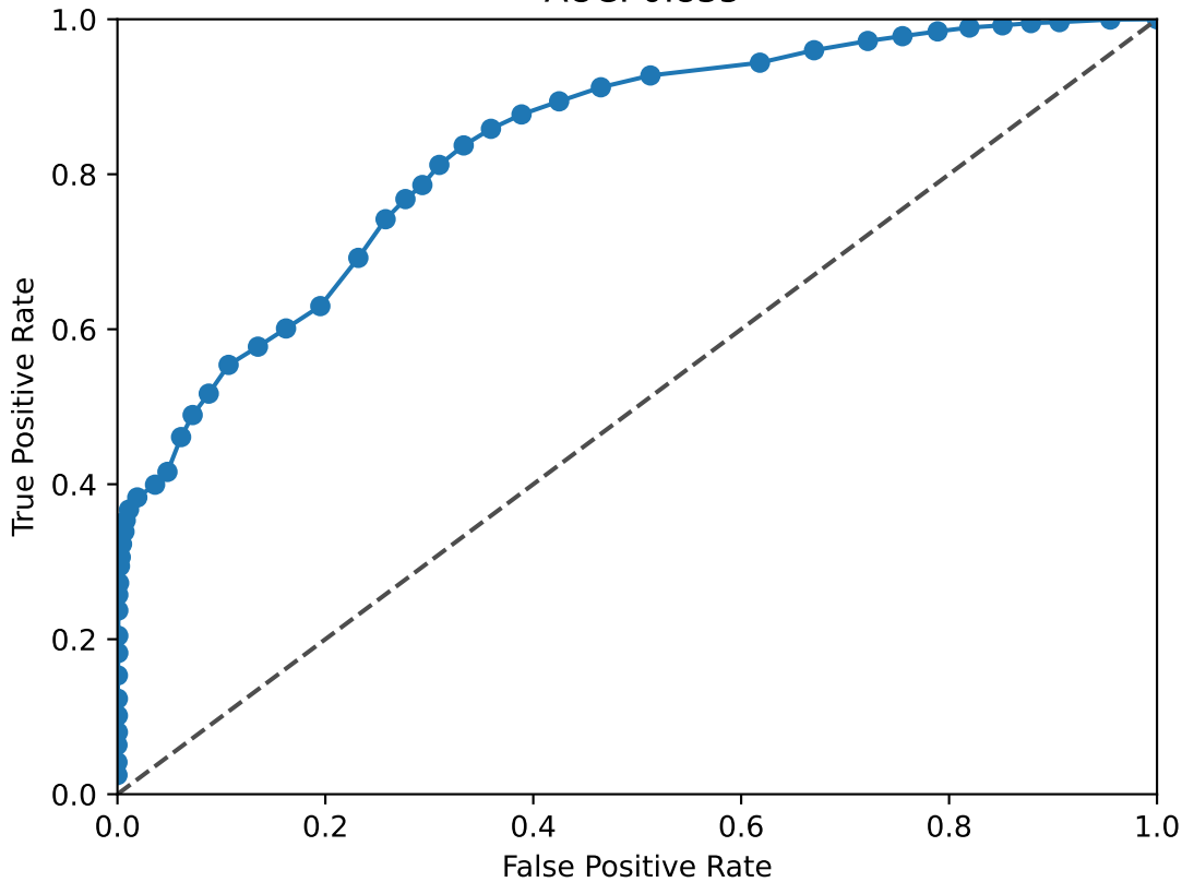
HES1 ROC Curve AUC: 0.835
