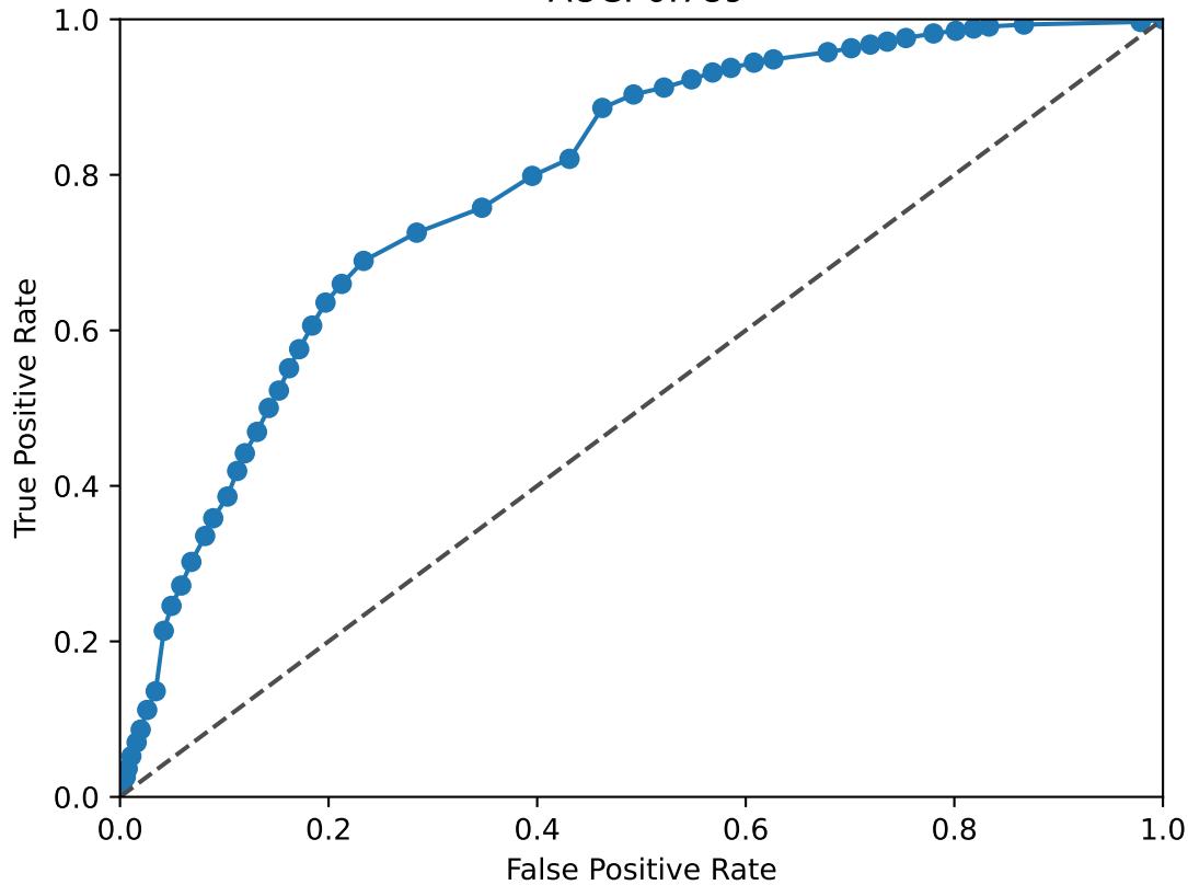
JUN ROC Curve AUC: 0.789
