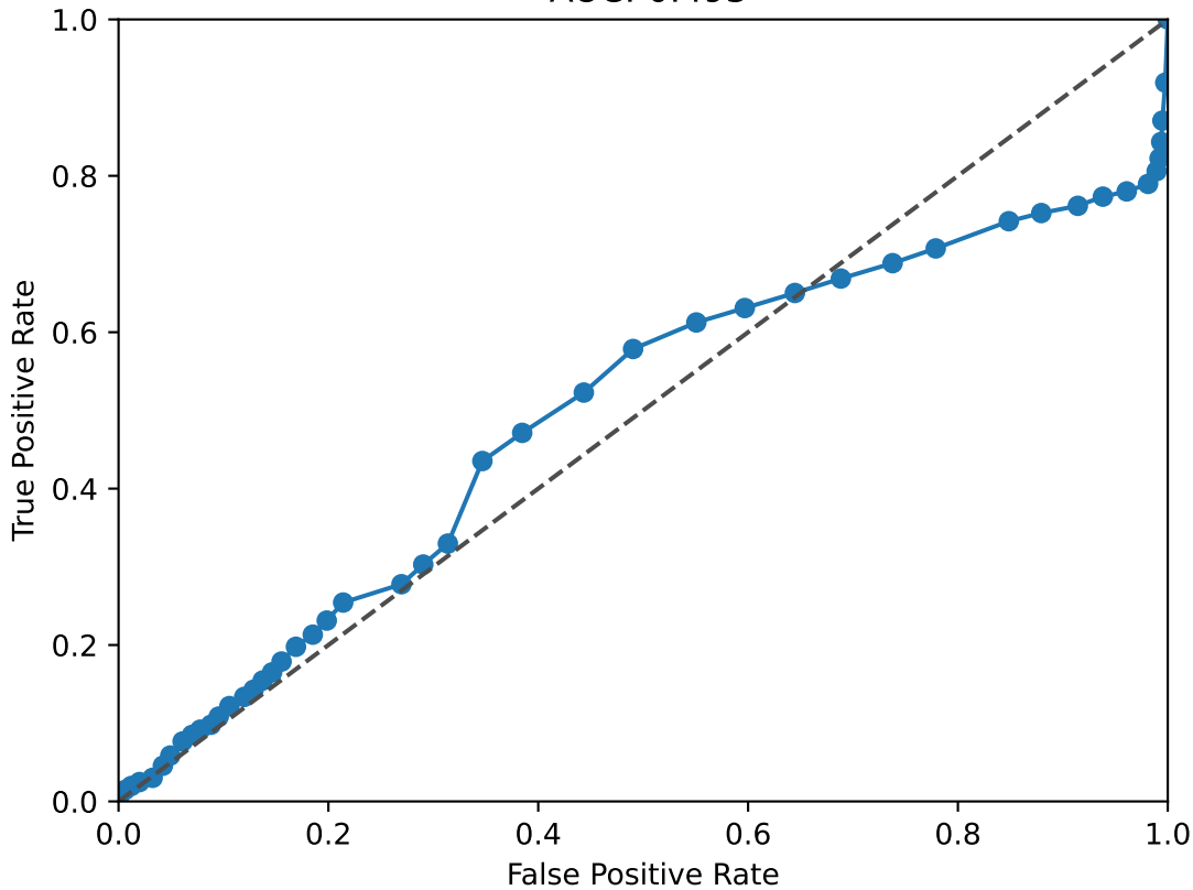
NFIX ROC Curve AUC: 0.493
