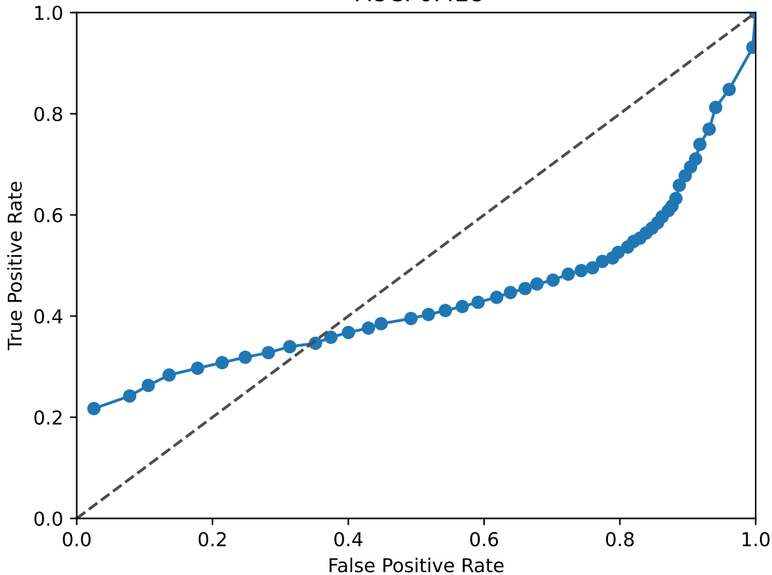
RORA_RORB ROC Curve AUC: 0.428
