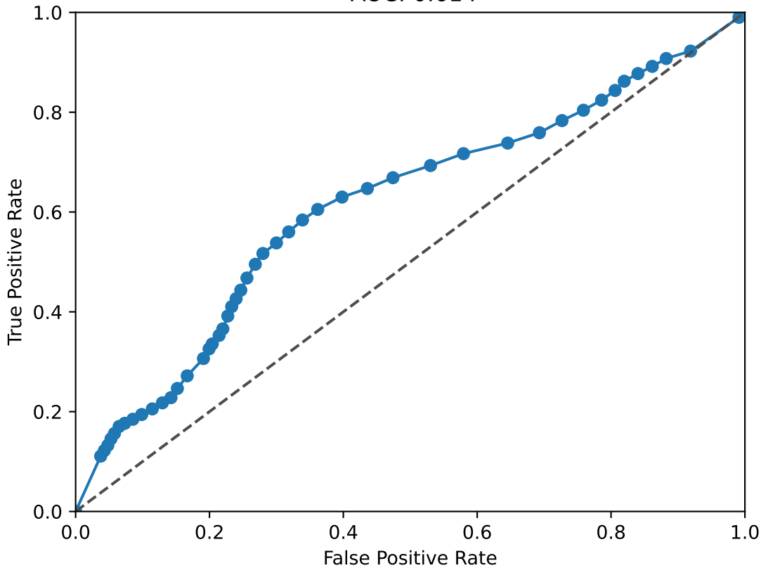
RUNX1 ROC Curve AUC: 0.614
