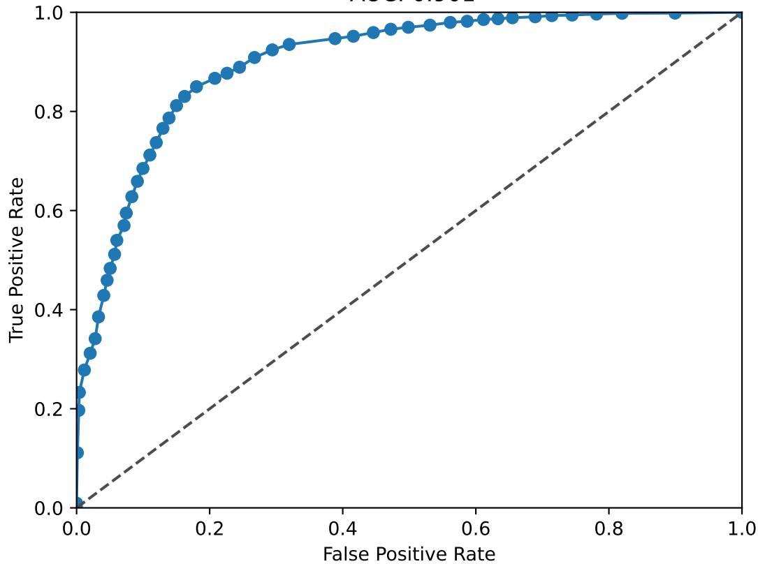
TEAD1 ROC Curve AUC: 0.901
