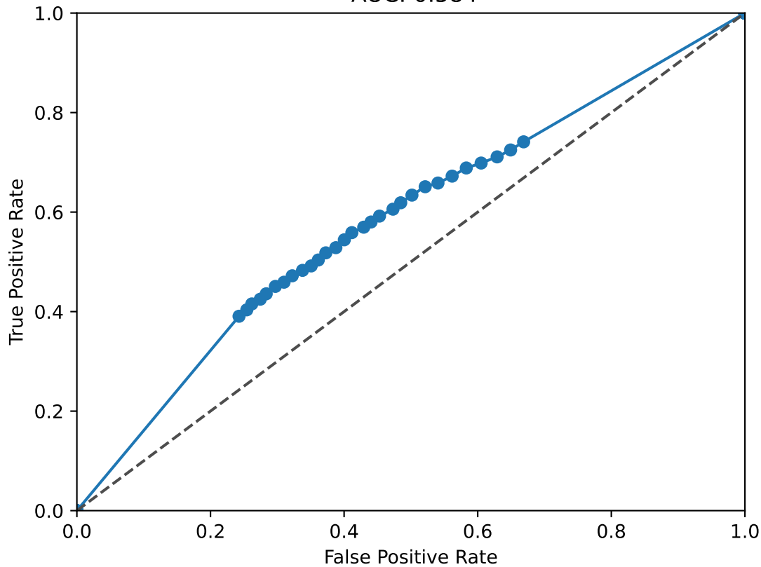
THR B ROC Curve AUC: 0.584
