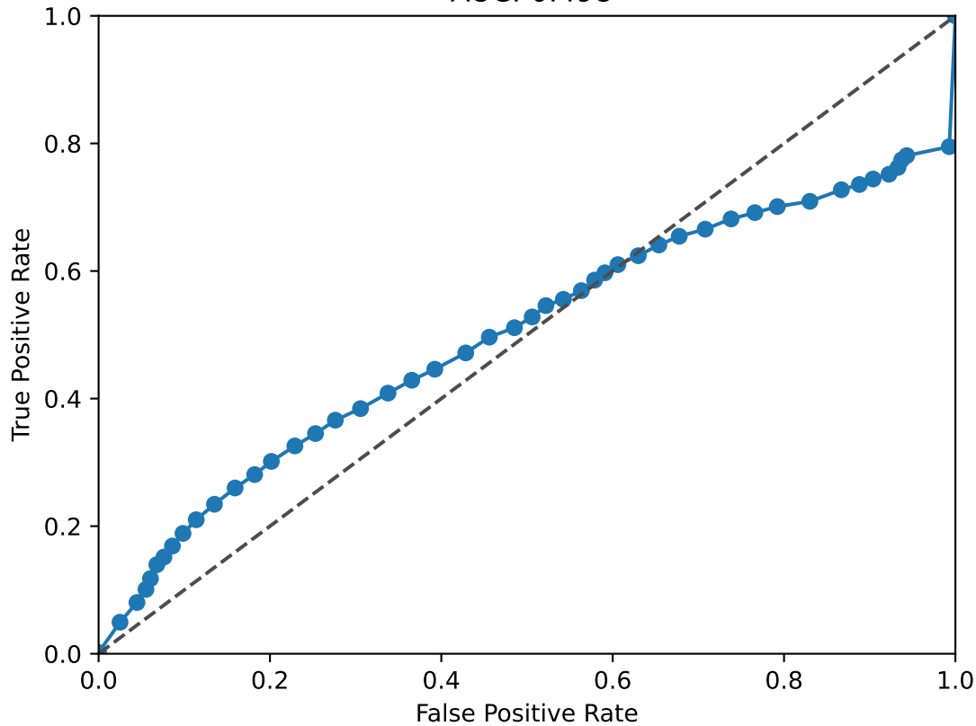
ASCL1 ROC Curve AUC: 0.498
