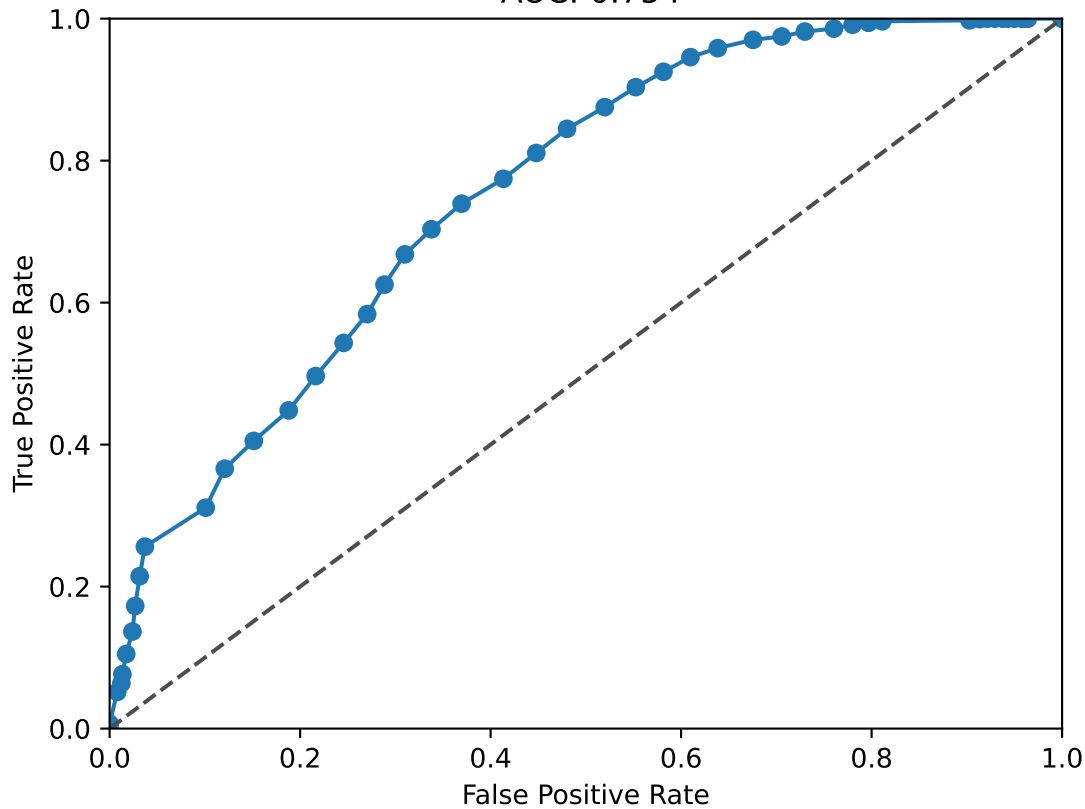
EGR1 ROC Curve AUC: 0.754
