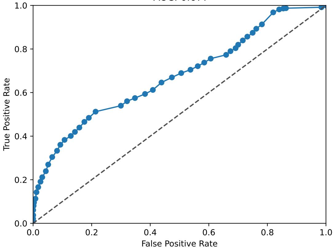
HES1 ROC Curve AUC: 0.677
