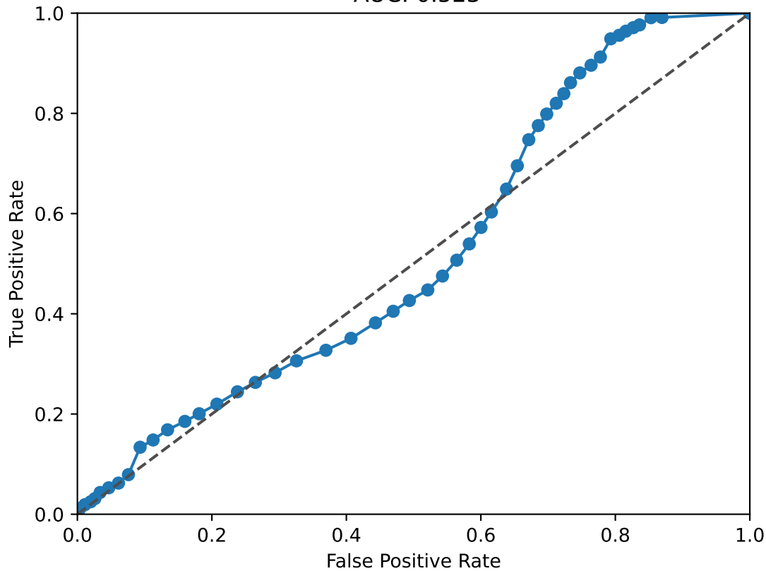
HSF2 ROC Curve AUC: 0.523
