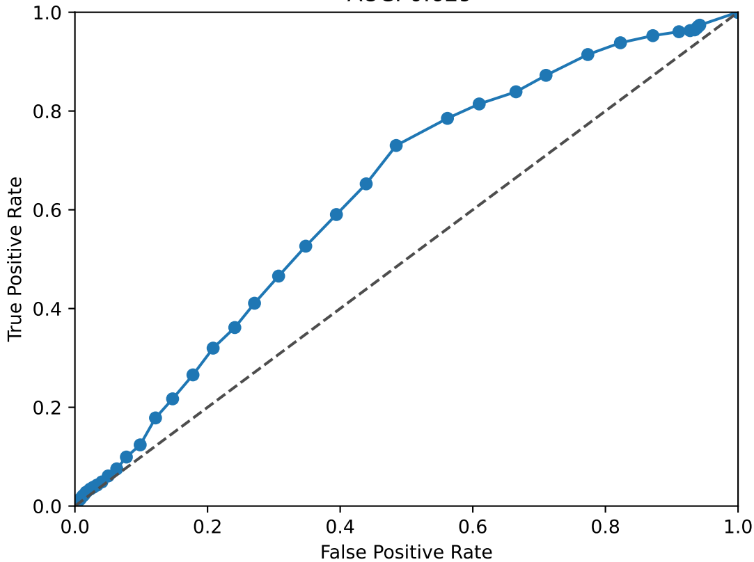
ICAM1 ROC Curve AUC: 0.629
