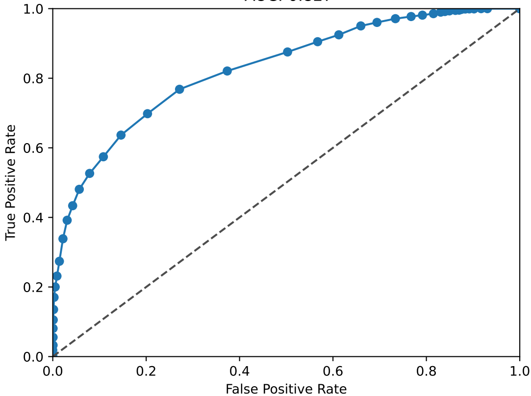
SIX4 ROC Curve AUC: 0.827
