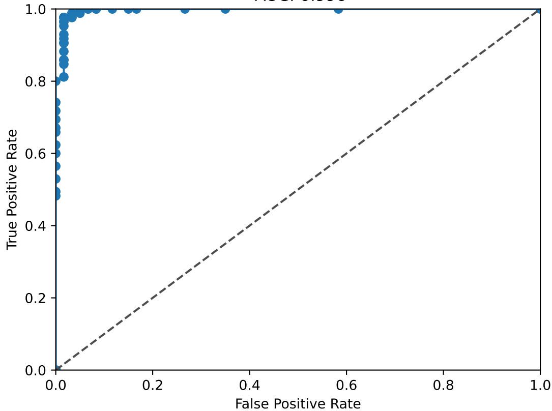
ASCL1 ROC Curve AUC: 0.996
