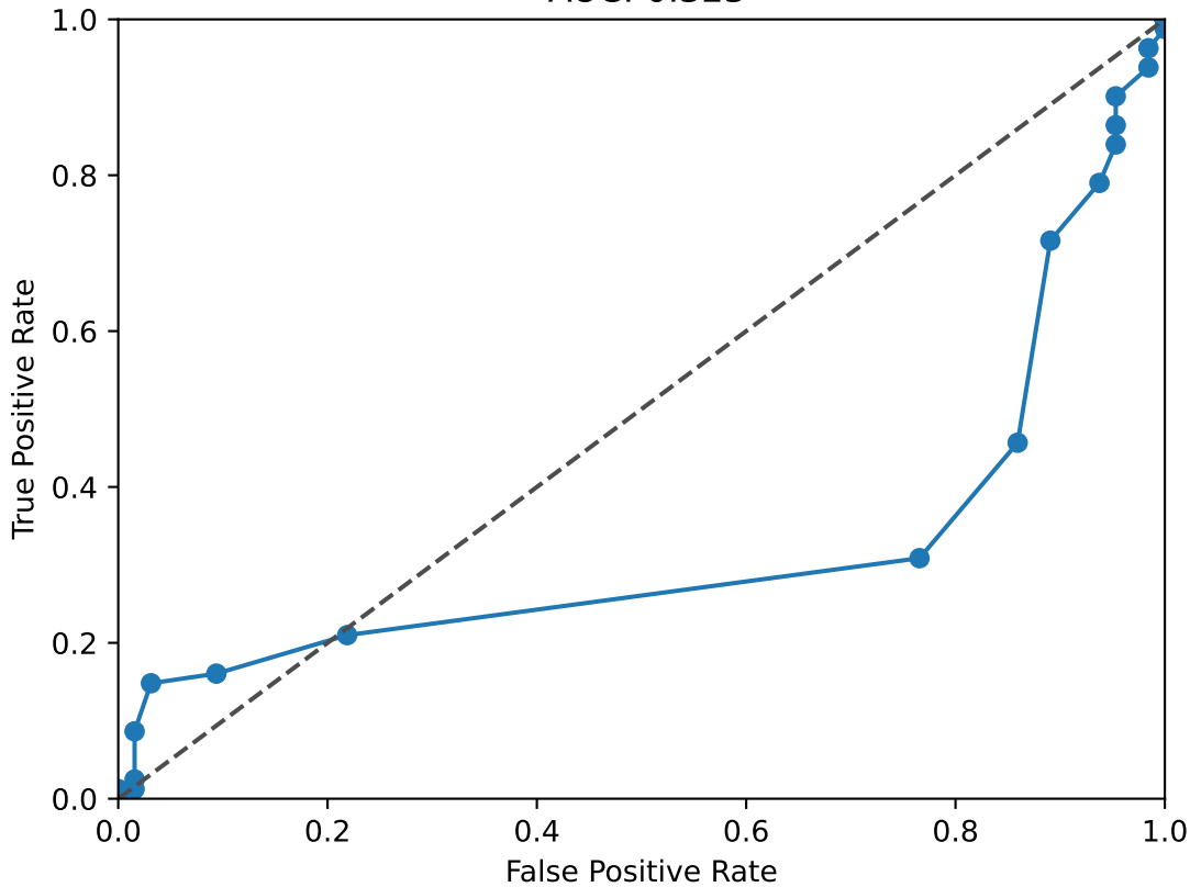
JUNB ROC Curve AUC: 0.323
