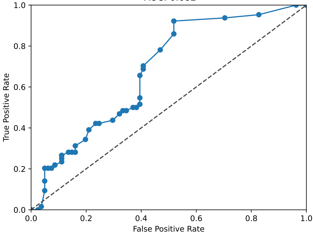
PKNOX2 ROC Curve AUC: 0.682
