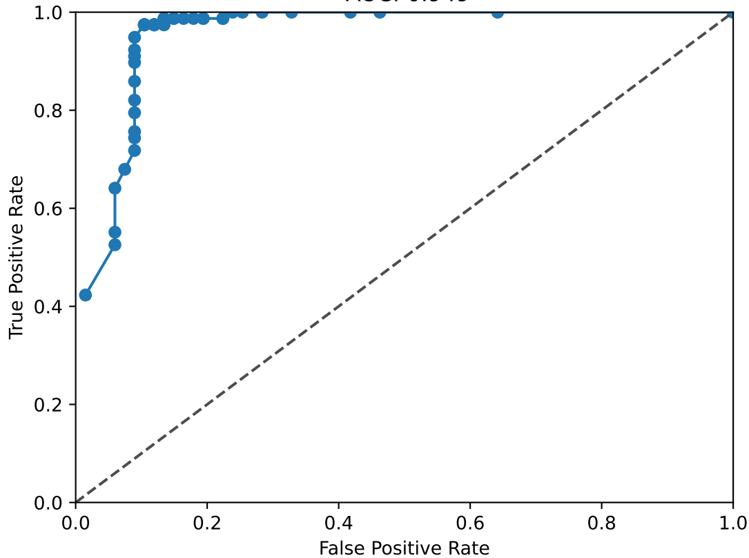
RORA_RORB ROC Curve AUC: 0.949
