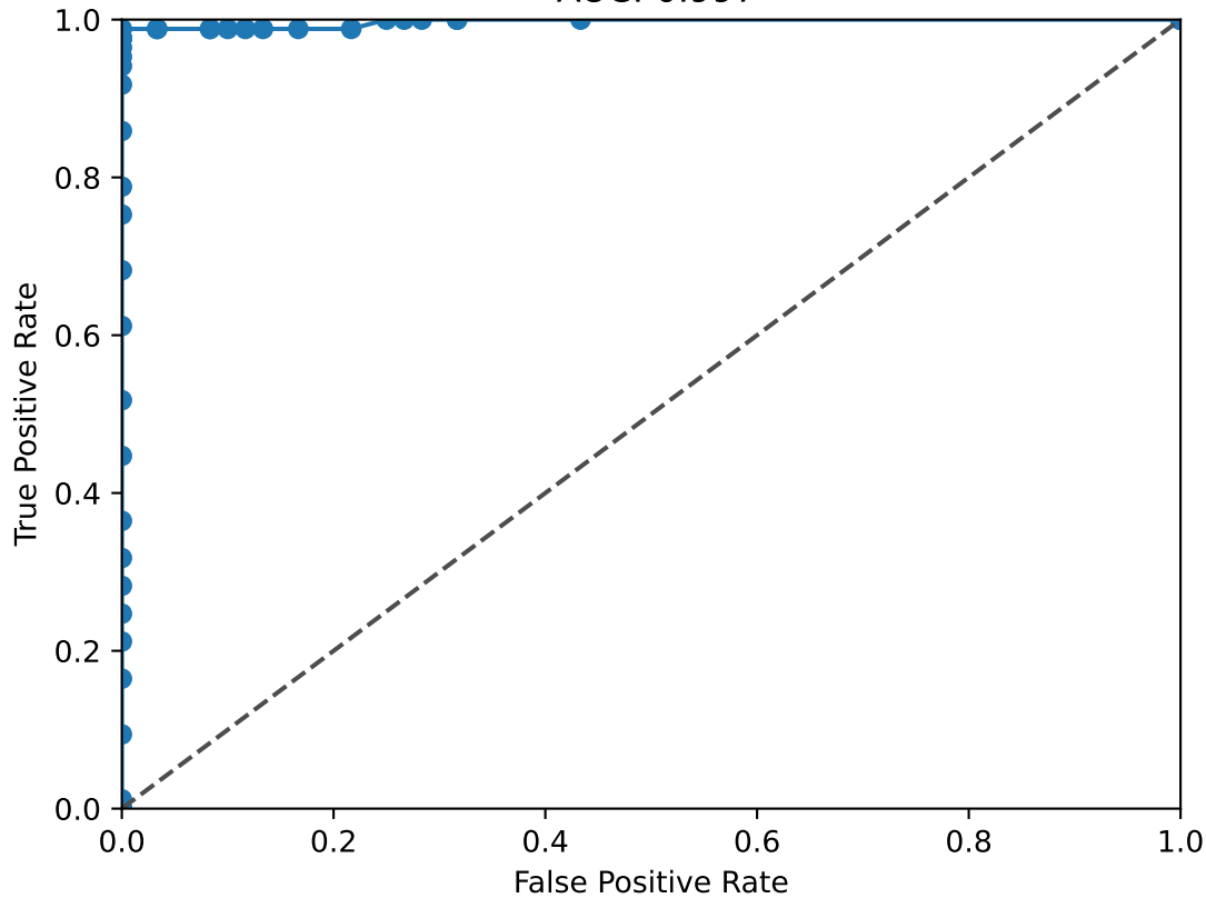
STAT2 ROC Curve AUC: 0.997
