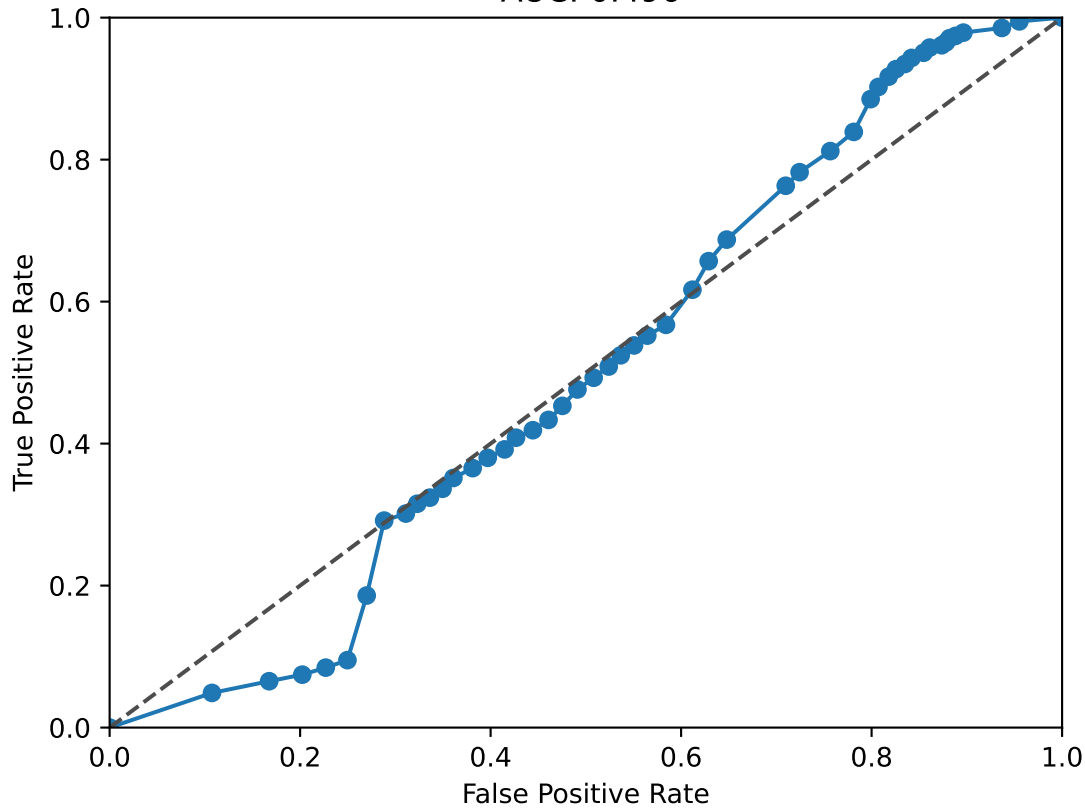
GRHL2 ROC Curve AUC: 0.496
