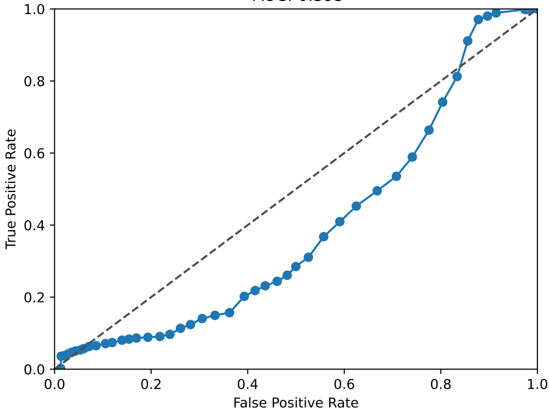
ICAM1 ROC Curve AUC: 0.395
