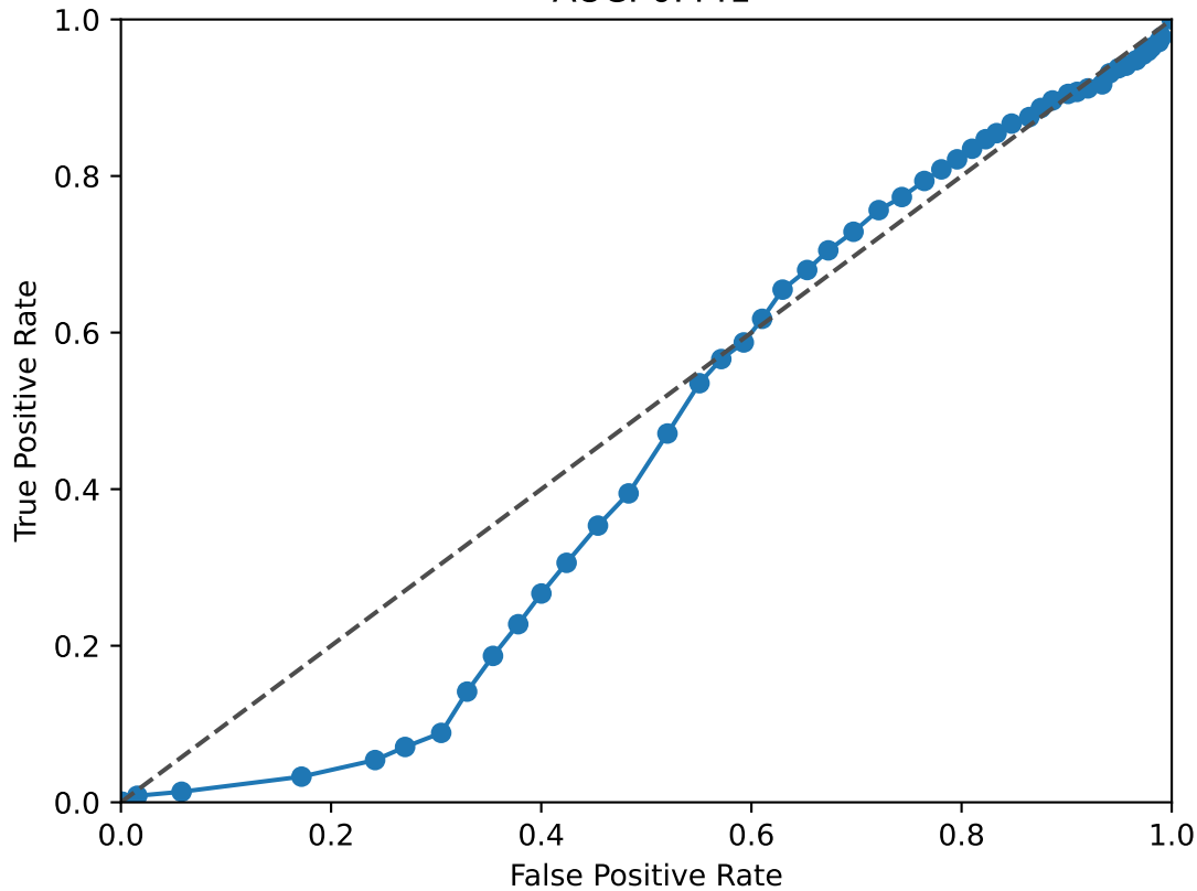
KMT2A ROC Curve AUC: 0.441
