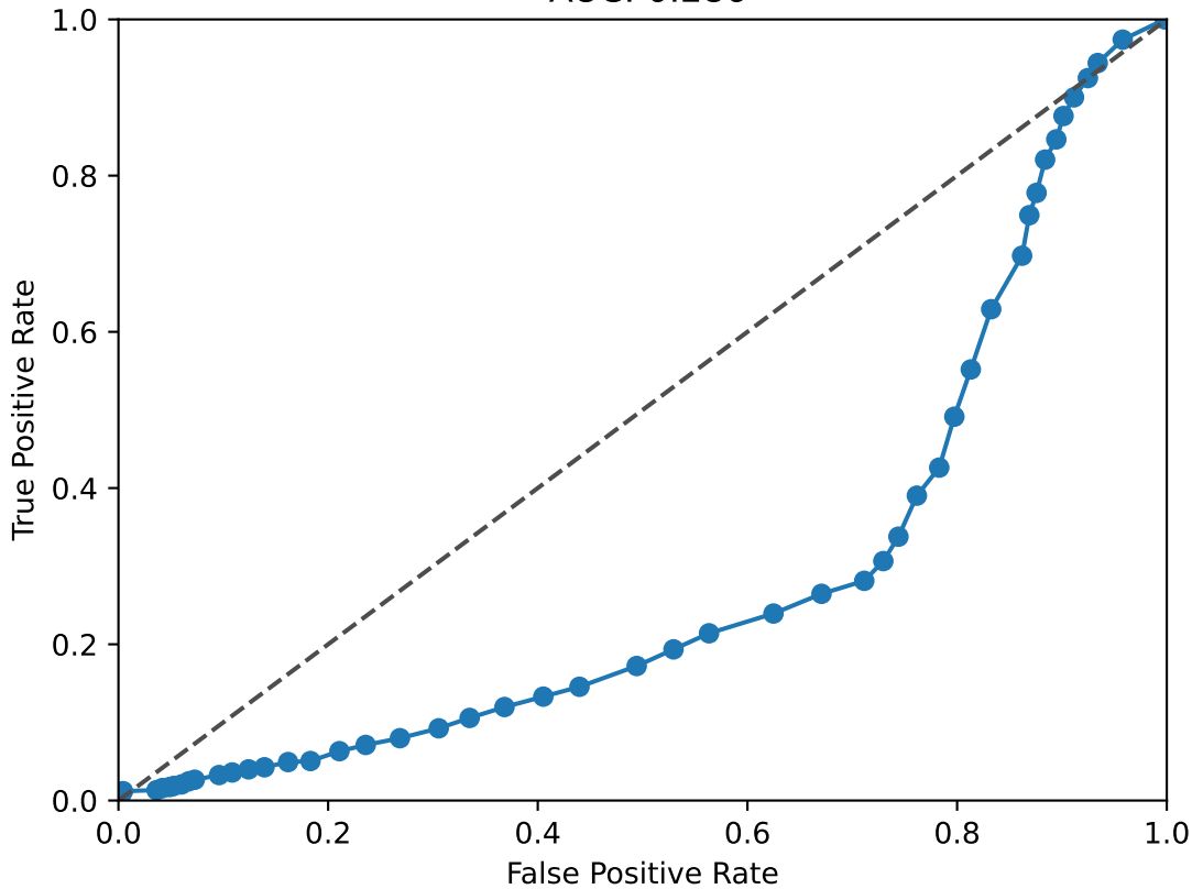
NFIX ROC Curve AUC: 0.286
