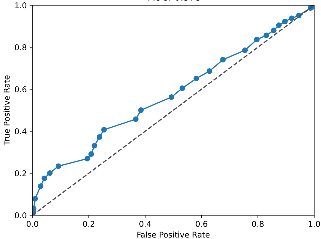
PBX1 ROC Curve AUC: 0.575
